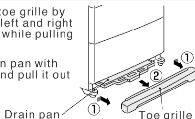
Drain pan Toe grille
